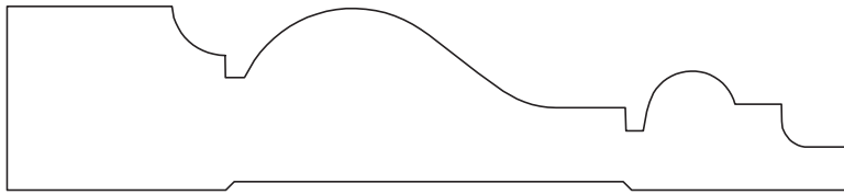
A&M # 3896 7/8" X 4"
