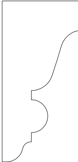
A&M # 5728 1-5/16" X 2-3/4"
