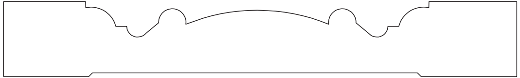
A&M # 2114 13/16" X 5-1/2"
