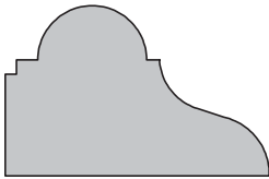
A&M # 7093 13/16 X 1-1/4"
