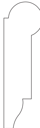
A&M # 8061 3/4" X 2-1/2"
