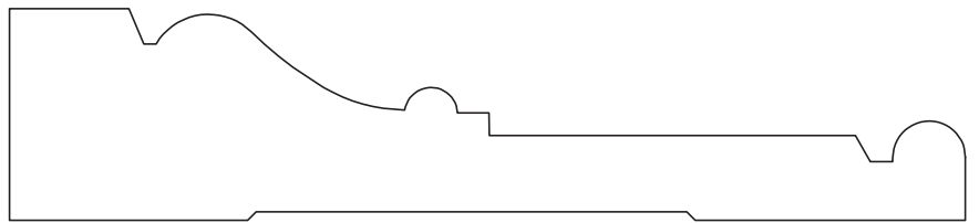
A&M # 3898 1" X 4-1/2"
