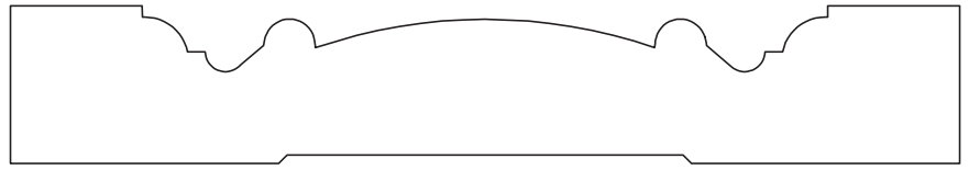
A&M # 2415 3/4" X 4-1/2"
