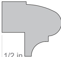
A&M # 4431 1-1/4" X 1-5/16" ALSO IN FIR
