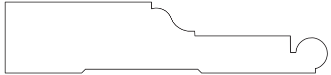
A&M # 3698 3/4" X 3-3/8"
