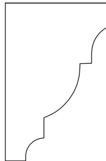
A&M # 19071 1-1/16" X 1-5/8"
