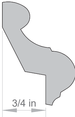
A&M # 1665 13/16" X 2"
