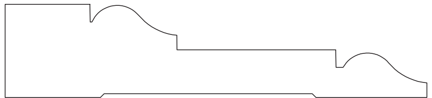
A&M # 30209 1" X 4-1/2"
