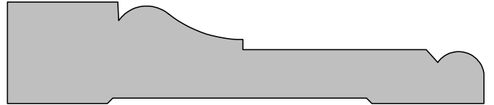
A&M # 3076 3/4" X 3-1/2"
