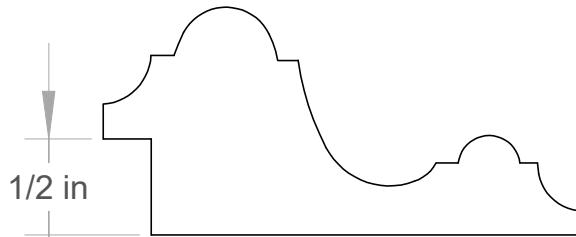
A&M # 7426 1-3/16" X 2-1/2"
