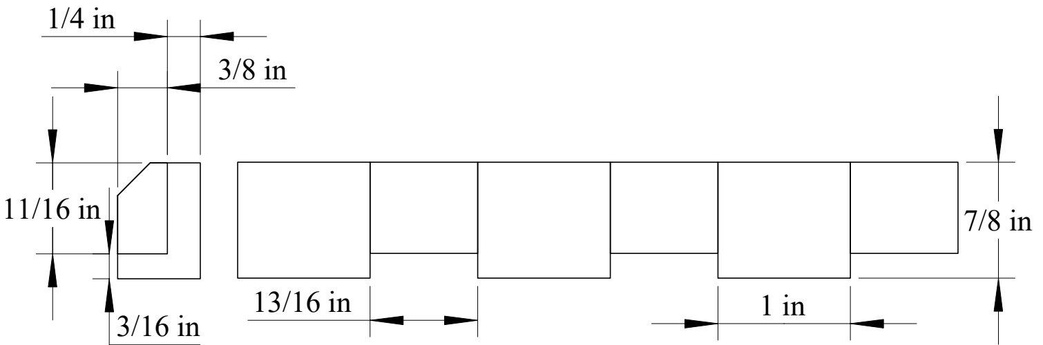
FRONT VIEW
