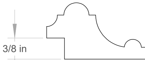
A&M # 7430 1" X 1-3/4"
