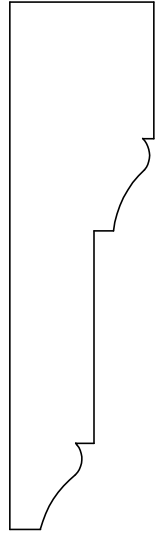
A&M # 4095 3/4" X 2-3/4"
