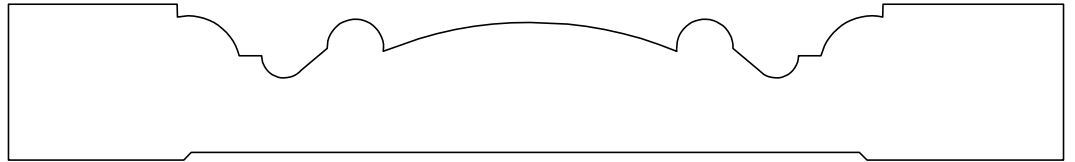
A&M # 2114 13/16" X 5-1/2"
