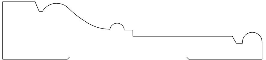
A&M # 3898 1" X 4-1/2"
