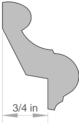
A&M # 1665 13/16" X 2"
