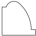
A&M # 7591 3/4" X 3/4"
