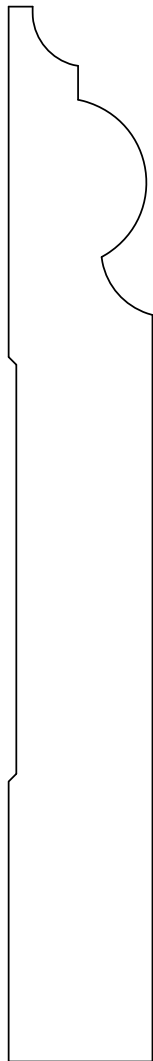
A&M # 18184 3/4" X 5-1/2"
